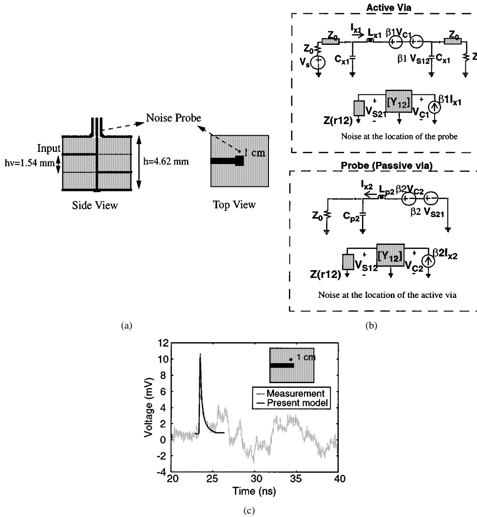
Fig. 9. (a) Stripline-via structure under test. The diameter of the via is 1 mm and the via pad is a 4 mm \times 4 mm square. The striplines are 2-mm wide, and \epsilon_r = 4 . (b) The developed model for the tested buried via structure. (c) Measured and simulated parallel-plate noise.
